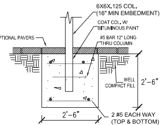
5 S1 COLUMN ATTACHED & ISOLATED FOOTING
