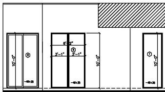
VIEW "B"
