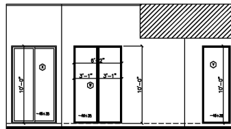
VIEW "A"
