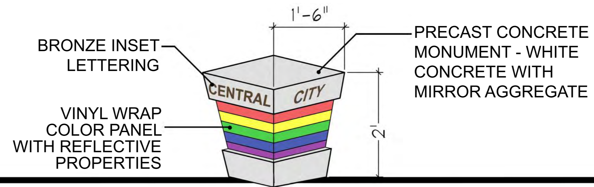
STREET END DISTRICT SIGN MONUMENT
