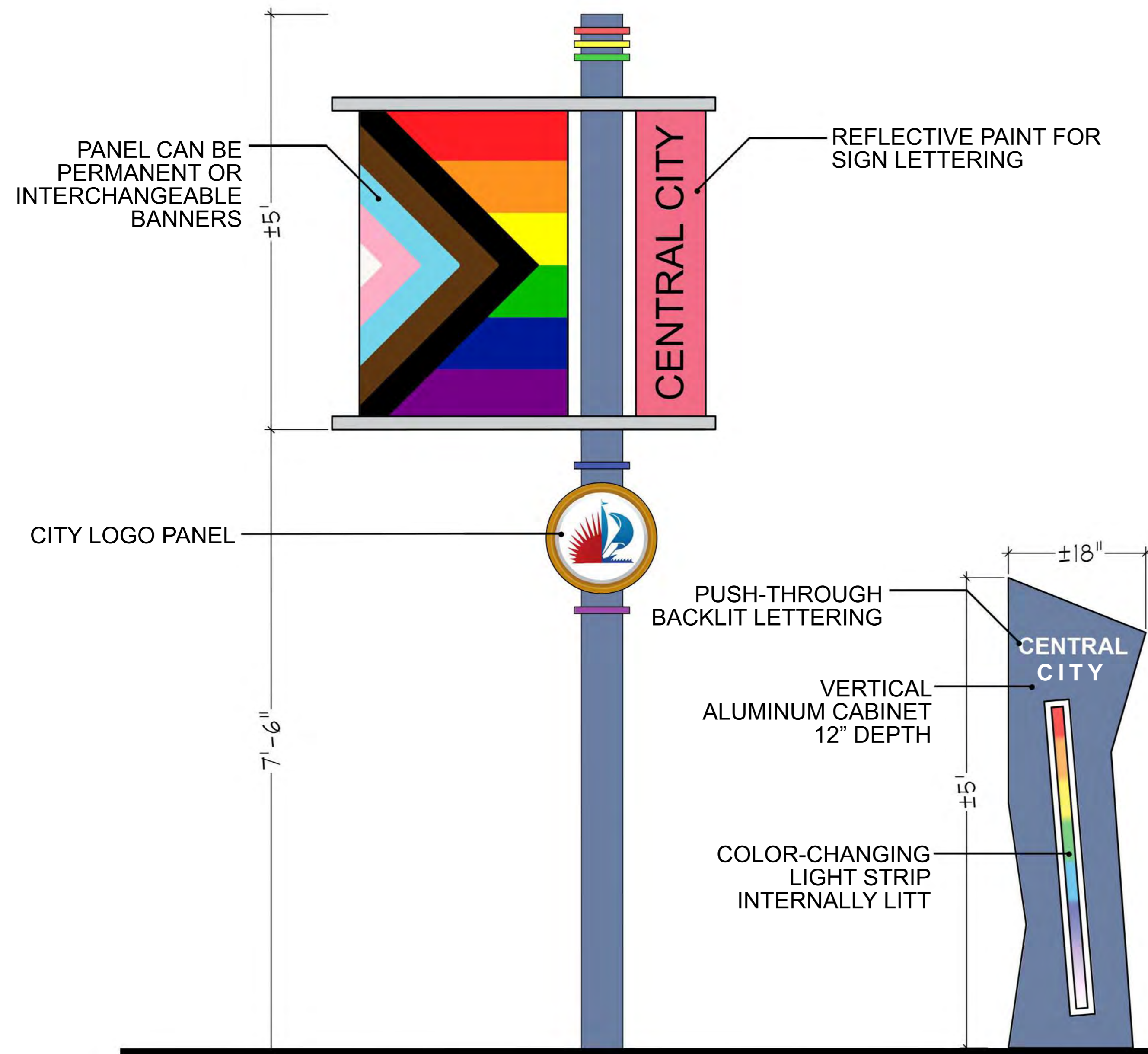
POST MOUNT DISTRICT SIGN
